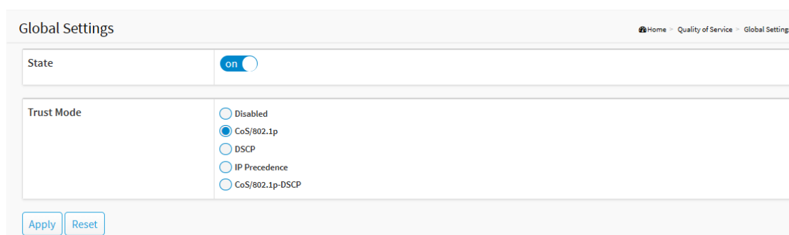
Figure 73: Global Setting
