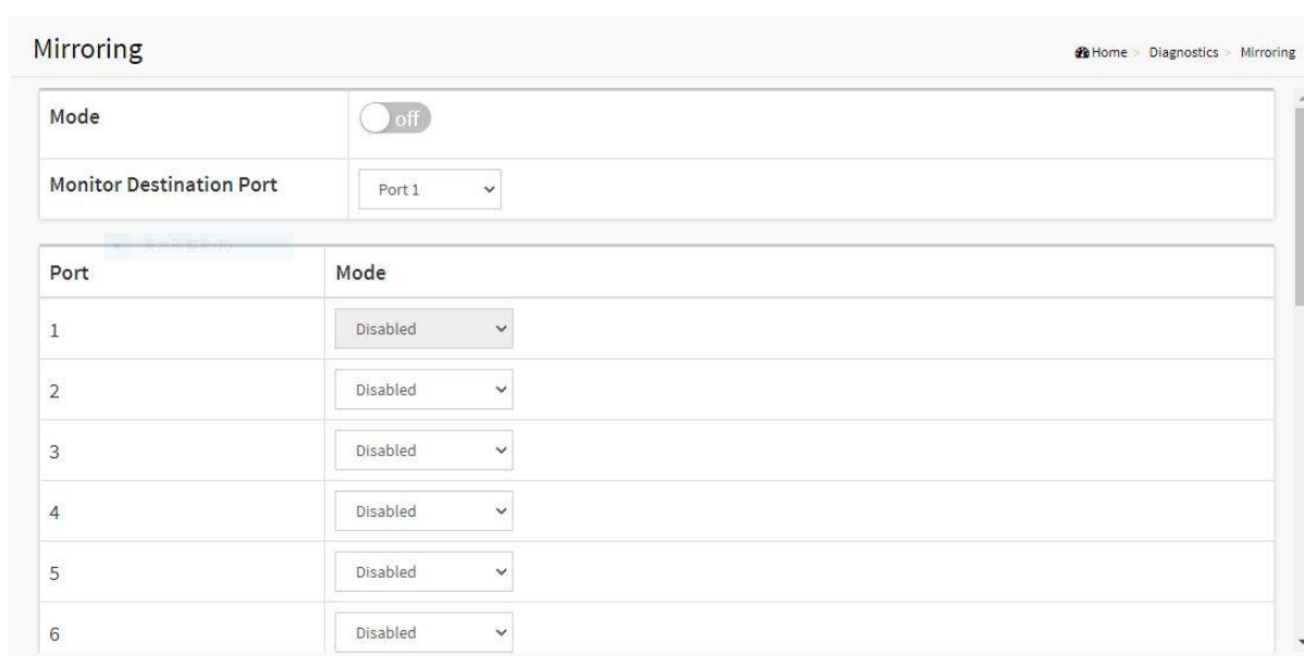
Figure 101: Mirroring
