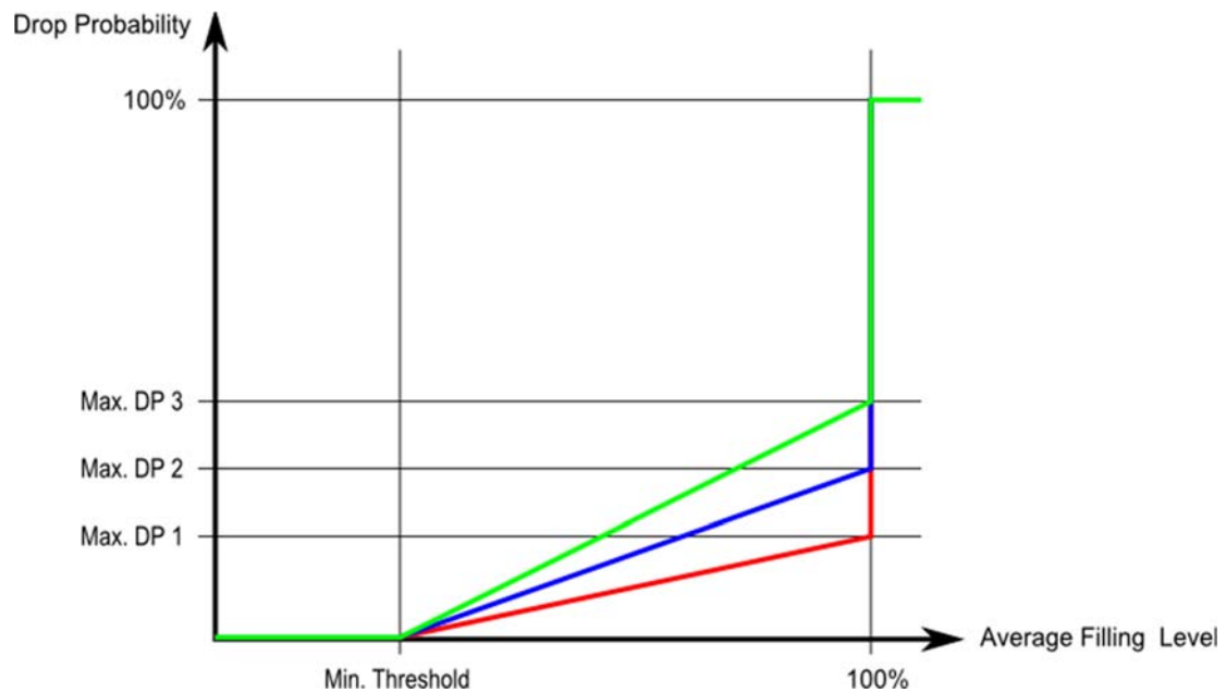
Figure 2-18.12: RED Drop Probability Function
