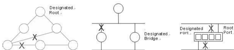
Figure 85: The Spanning Tree Protocol
