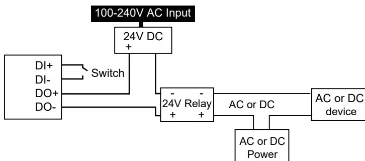
DI/DO Connection Diagram w/ AC or DC Relay
